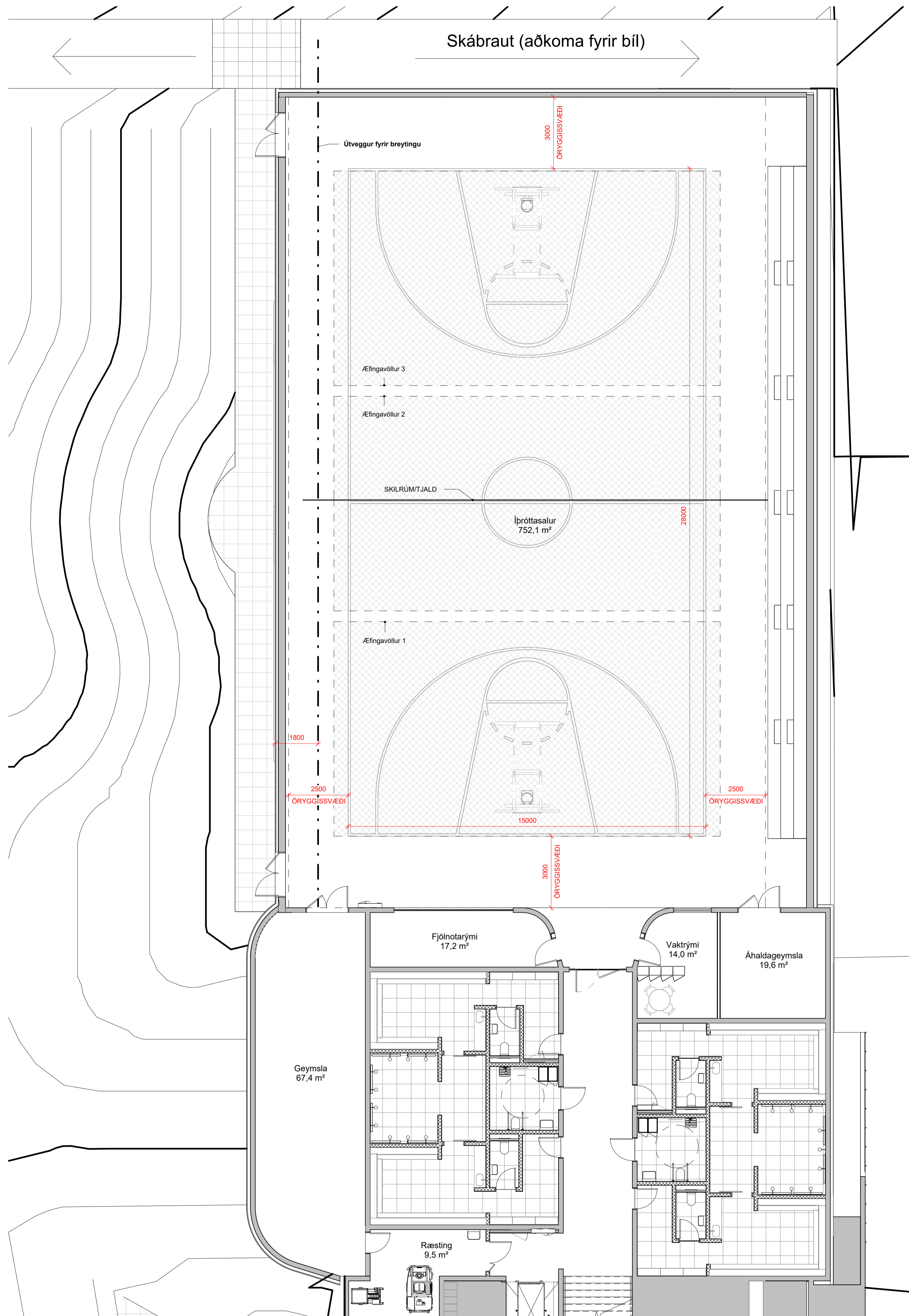
1 S-128 - ÍÞRÓTTAHÚS BREYTINGARTILLAGA 1 : 100
